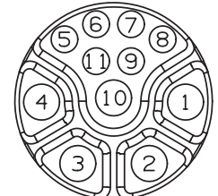
CONTACT VIEW
