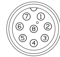
CONTACT END VIEW
