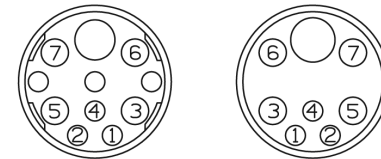
7 PIN FEMALE CONNECTOR
